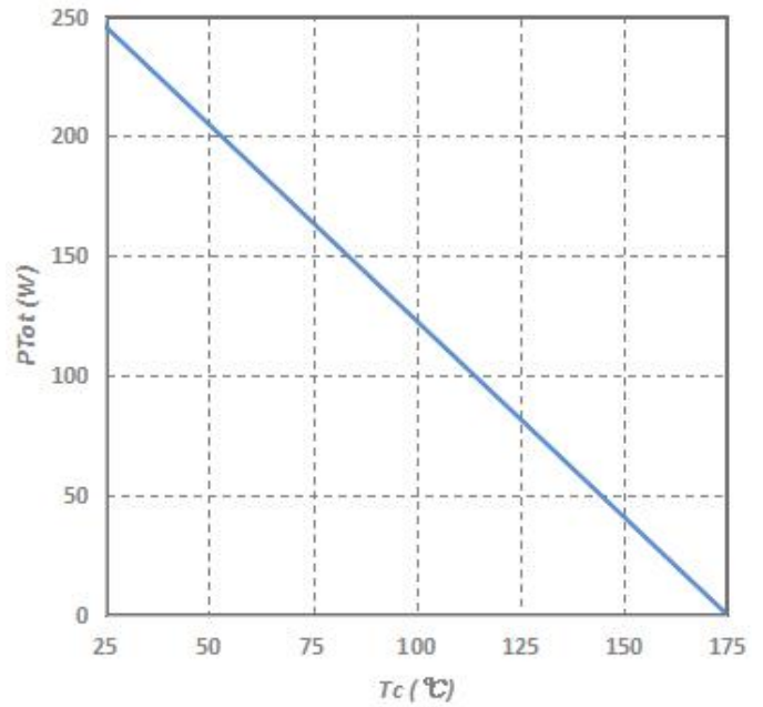
Fig.6-Power Derating
